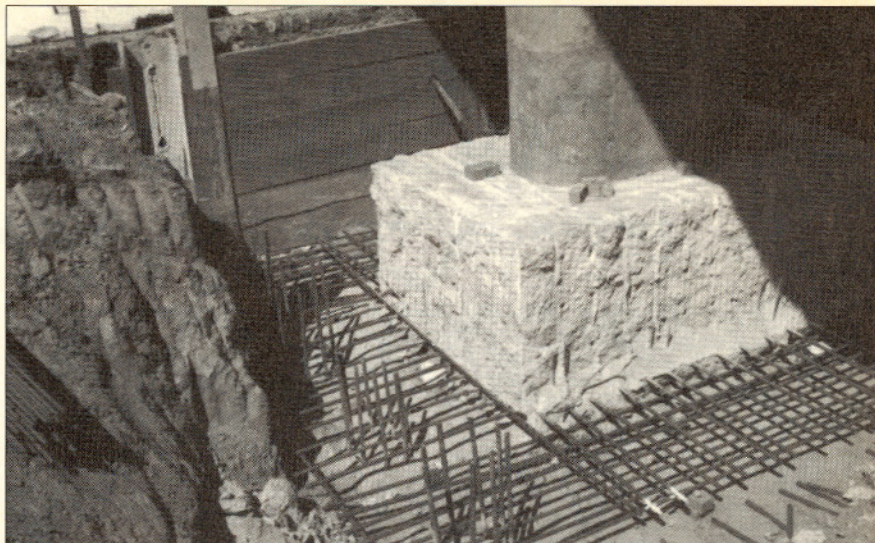
A view of a footing after the outer edges have been removed and the mat rebar welded to the base of the rebar cage for the new footing. The tops of the concrete cast-in-drilled-hole pilings are visible along the left side of the footing.
